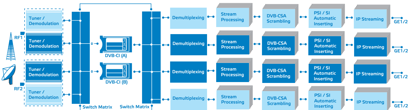
Block Diagram, Dual / Quad Receivers (only Quad C, T/T2 and ISDB-T Receivers)
