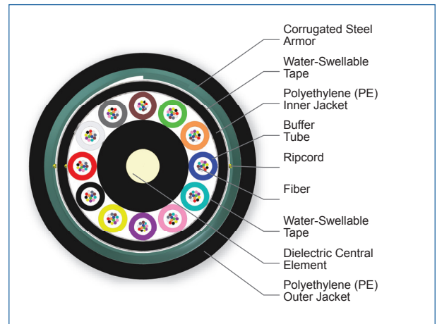
Cross Section of Part Number: 144EU5-T4101F20
