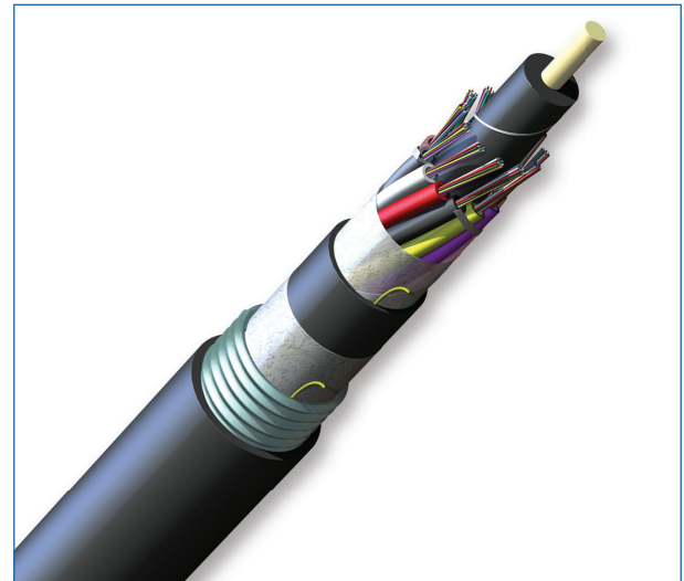
Part Number: 144EU5-T4101F20
